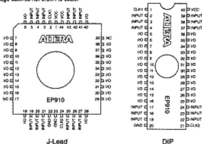
Figure 7. EP910 Package Pin-Out Diagrams
